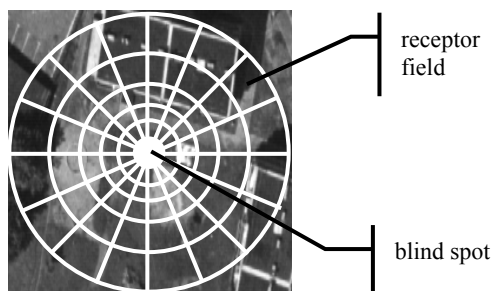
Figure 2. Distribution of receptor fields in the log-polar transformation
