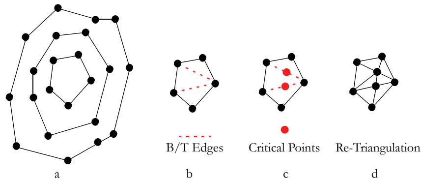
Figure 22-4 a: Contours at the top of a hill; b: triangulation of highest contour, with B/T edges identified; c: placement of critical points on B/T edges; d: re-triangulation
