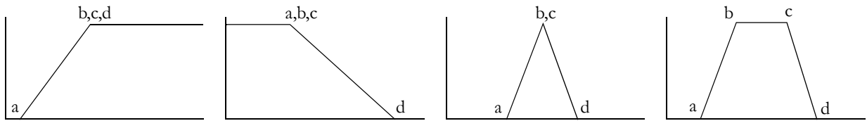
Figure 13-9 Linear Membership Function
