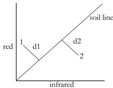
Figure 18-5 Distance from the Soil Line
