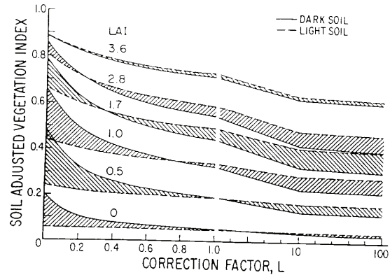
Figure 18-6 Influence of light and dark soil on the SAVI values of cotton as a function of the shifted correction factor L (from Huete, 1988).
