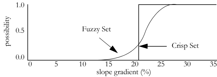
Figure 13-6 Fuzzy vs. Crisp Set Membership Functions
