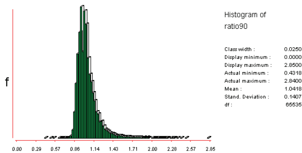
Figure 18-2 Histogram of a RATIO VI Image
