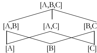
Figure 13-11 Hierarchical Structure of the Subsets in the Whole Set [A,B,C]
