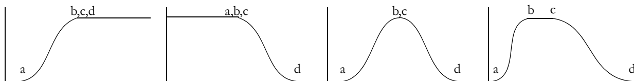
Figure13-7 Sigmoidal Membership Function
