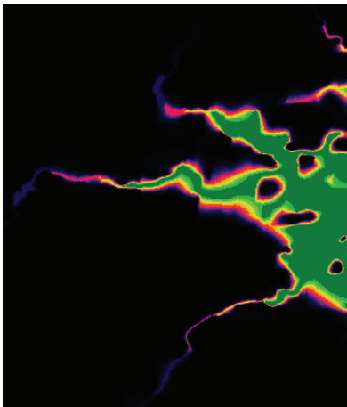
Figure 13-3 Probability of being flooded.
