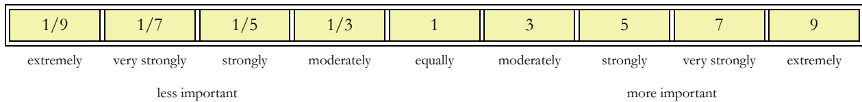
Figure 12-2 The Continuous Rating Scale
