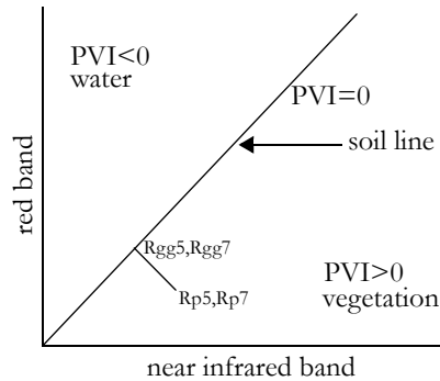
Figure 18-4 The Perpendicular Vegetation Index (from Richardson and Wiegand, 1977)
