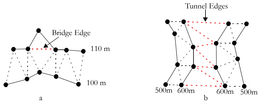
Figure 22-5 a: Contours at a stream; b: contours at a “saddle” feature. Contours are shown with solid lines, constrained triangle edges with dashed lines. B/T edges are shown in red.
