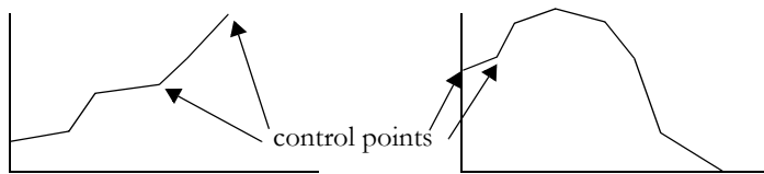
Figure 13-10 User-Defined Membership Function
