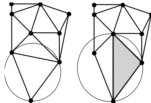
Figure 22-2 Delaunay triangulation (left) and non-Delaunay triangulation (right). The shaded triangle doesn't meet the empty circumcircle criterion.
