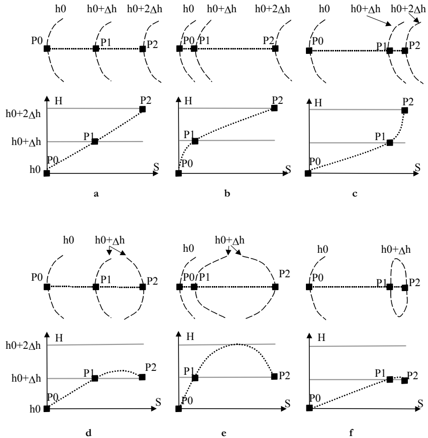
Figure 22-8 Six examples of parabolic critical point interpolation. The upper part of each example illustrates the map view of the isolines (dashed) and the intersection points (P0, P1 and P2) for one search direction (dotted line) for a critical point. The lower part shows the parabola for that set of intersection points. The attribute for the critical point (which is always between P1 and P2) can be found by plotting the critical point on the parabolic curve at its distance (S) from P0.
