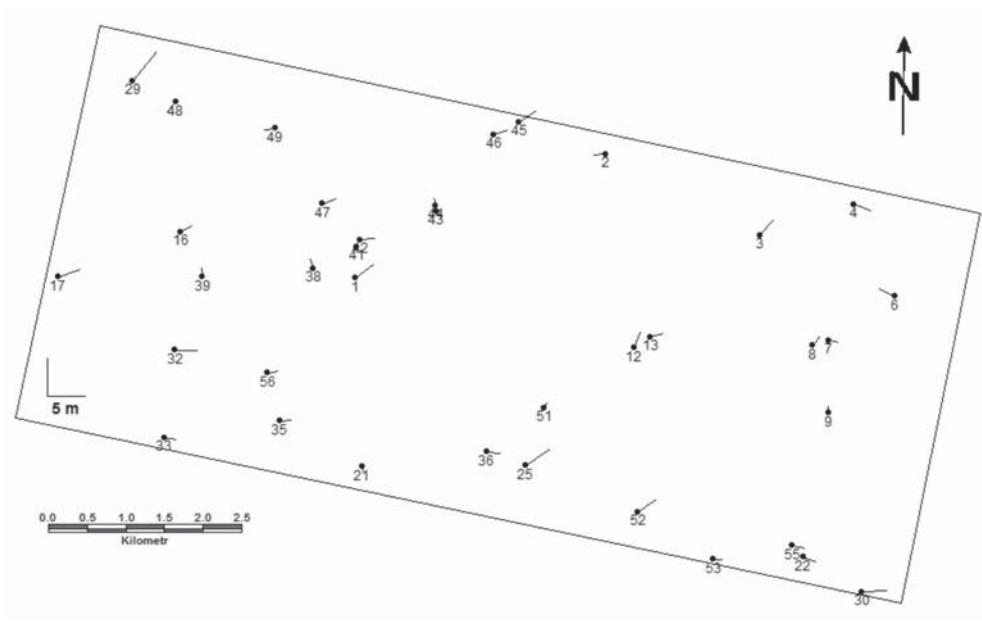
Fig. 4. Check points deviations for TSX-2 orthoimage generated based on one point and DEM LPIS model
